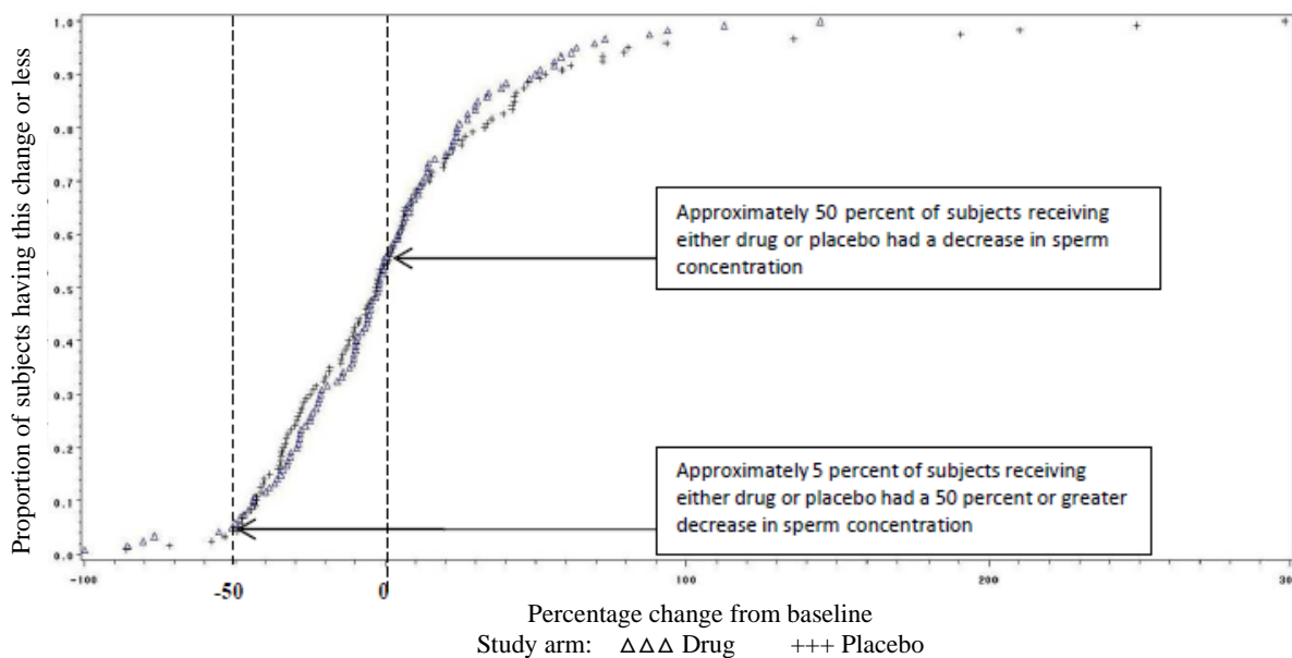
Figure 1. Example of a Cumulative Distribution Plot
